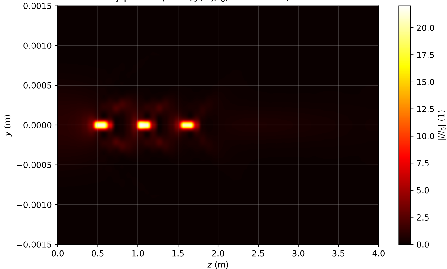
Intensity profile I(x=0, y, z)/I_0 , P_{in}=5.0P_{cr} , artificial time
